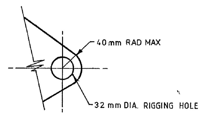
DETAIL OF RIGGING ATTACHMENT POINTS
