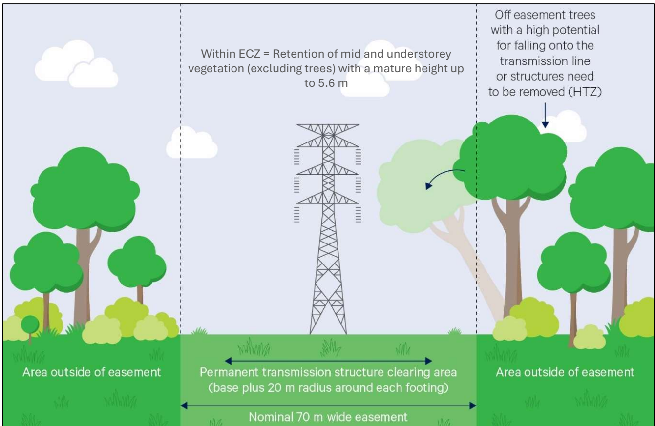
Plate 3-2 Indicative vegetation clearing around a typical transmission line structure
