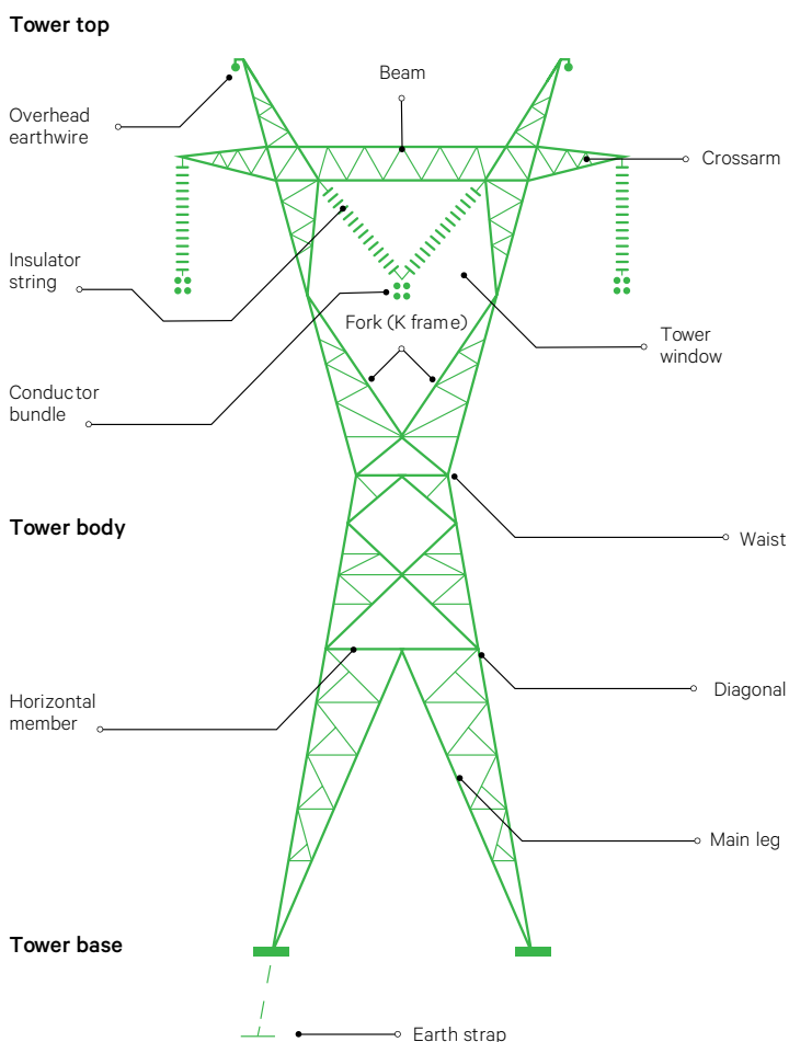
Figure 2: Example transmission tower
