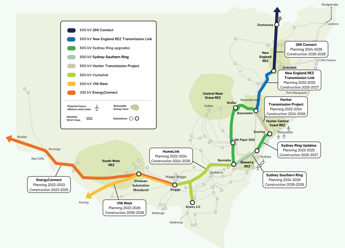
Figure 2: Transgrid's transmission infrastructure in NSW over the next decade.
