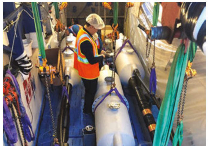
電纜接駁和調試 (Rawson Road接駁井, Greenacre)
