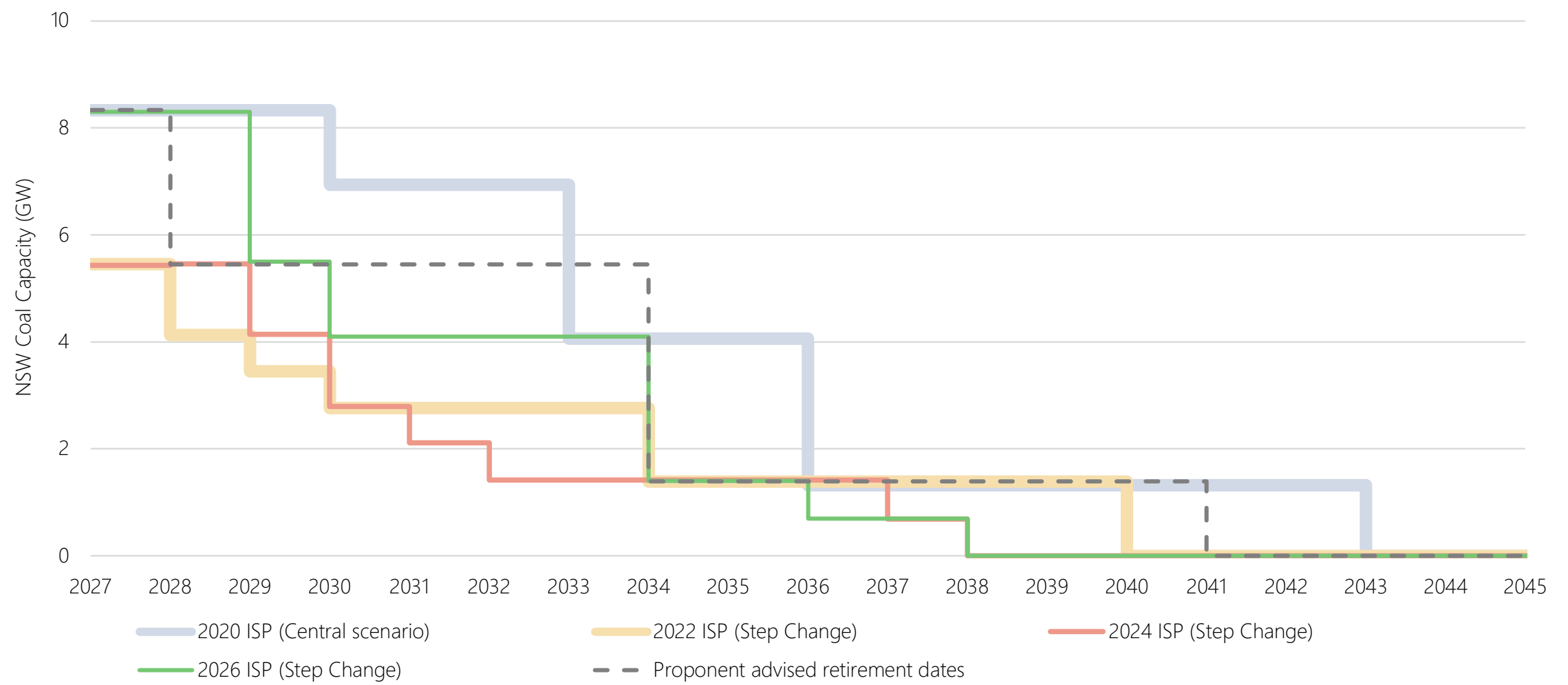
Figure 5.1: Capacity of coal generators available in NSW, based on projected retirement dates
