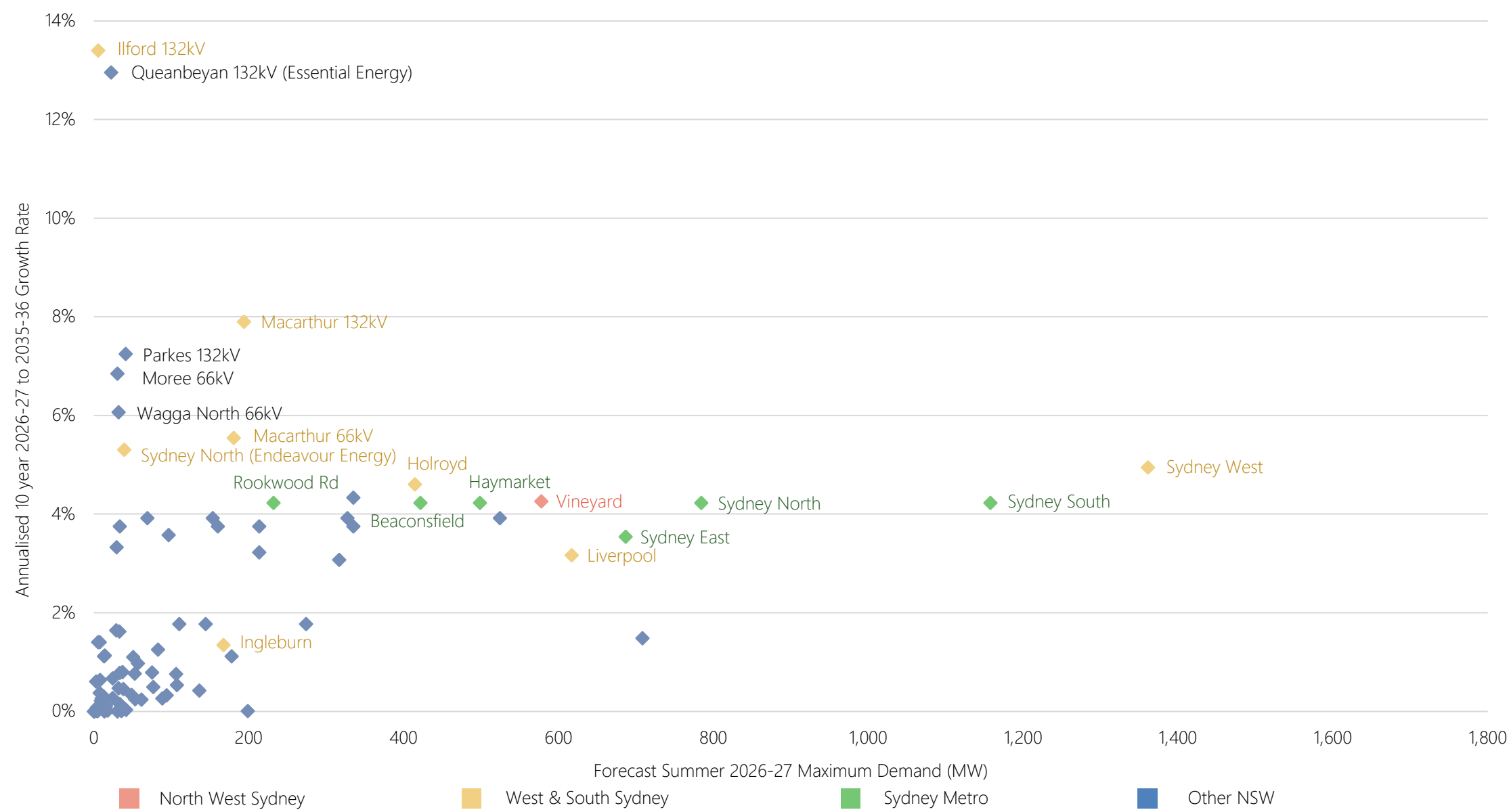
Figure 4.8: BSP forecast growth rates (Summer)
