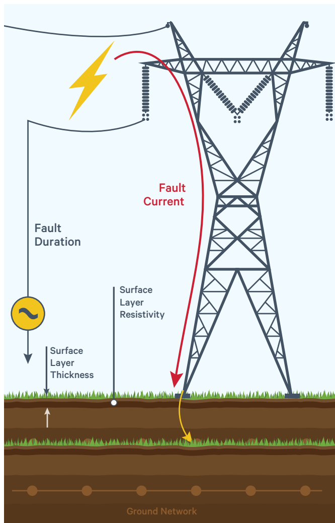
Figure 2: Earth potential rise
