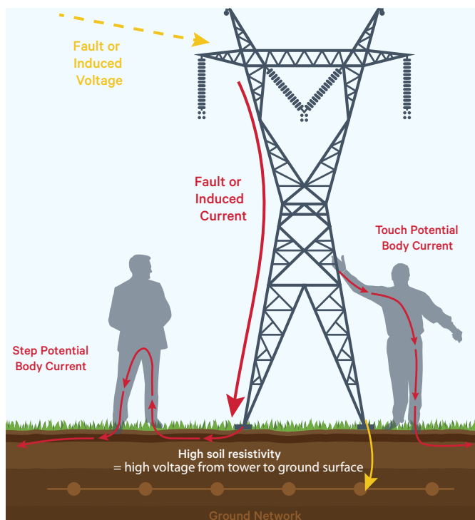
Figure 3: Touch and step voltages
